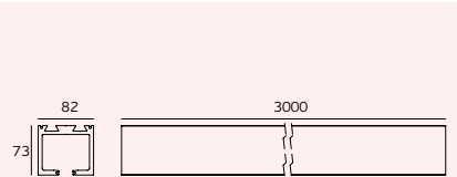
IN.15.551 Carril superior (3000mm) / Upper track (3000mm) / Carril superior (3000mm).
