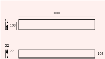
IN.15.550 Calha superior / inferior 1000mm Lower and uper track 1000mm Perfil inferior y superior 1000mm.
