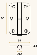
SM.005.A.ECO Dobradiça / Flat hinge / Bisagra plana.
