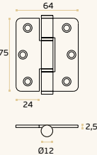
SM.005.D.ECO Dobradiça / Flat hinge / Bisagra plana.
