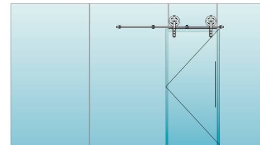
(B) FIXED AT GLASS / CARRIL / RAIL FIXO NO VIDRO 1900mm
