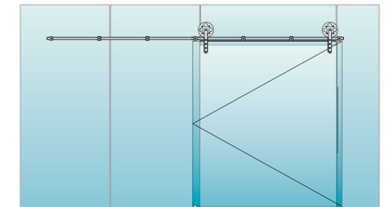
(B) FIXO NO VIDRO / CARRIL / RAIL FIXED AT GLASS / FIJA EN Cristal 3700mm
