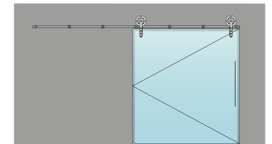
(A) FIXAÇÃO À PAREDE / CARRIL / RAIL FIXED AT WALL / FIJADO A PARED 3700mm
