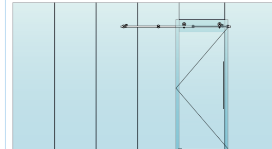
(C) FIXO NO VIDRO / FIXED AT GLASS / FIJO EN CRISTAL CARRIL / RAIL 1900mm
